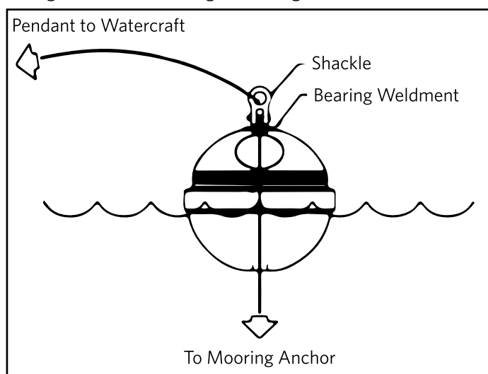
Diagram B: Pass-Through Mooring Hardware Installation
