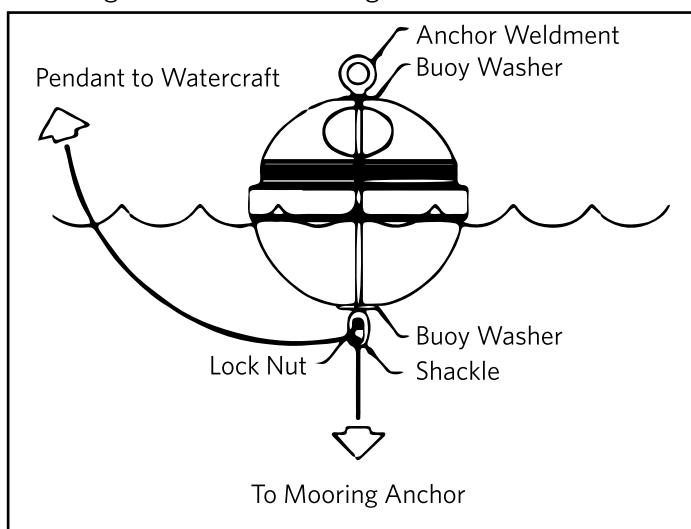
Diagram A: Fixed Mooring Hardware Installation
